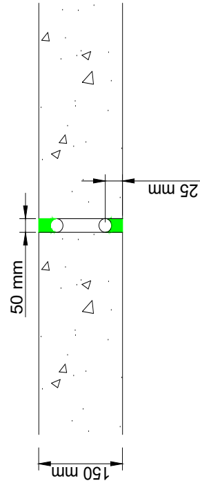
Rigid floor seal with polyethylene backing rod
