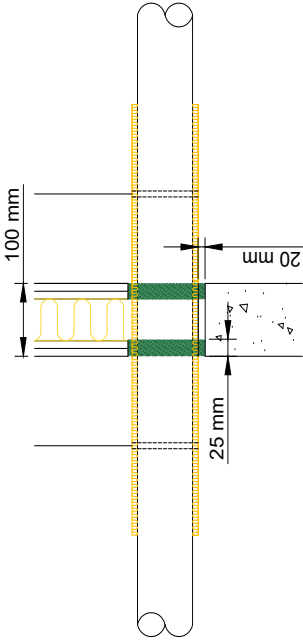
Insulated copper/metal/steel pipe rigid floor with Stonewool 45kg/m³ density backing
