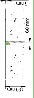
Rigid floor single seal with steel from above with stonewool backing
