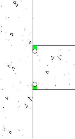
Concrete/Blockwork rigid wall seals polyethylene backing
