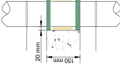
Combustible pipe rigid floor with Stonewool 45kg/m³ density backing
