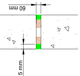
Typical hardwood and softwood rigid wall with stonewool backing
